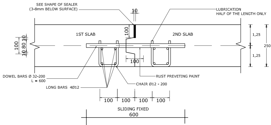
CONSTRUCTION JOINT MELINTANG SKALA 1:10
