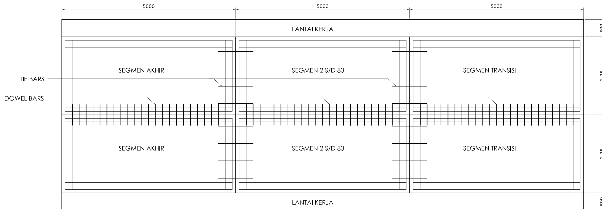
LAYOUT SEGMENT TIE BARS DAN DOWEL BARS
