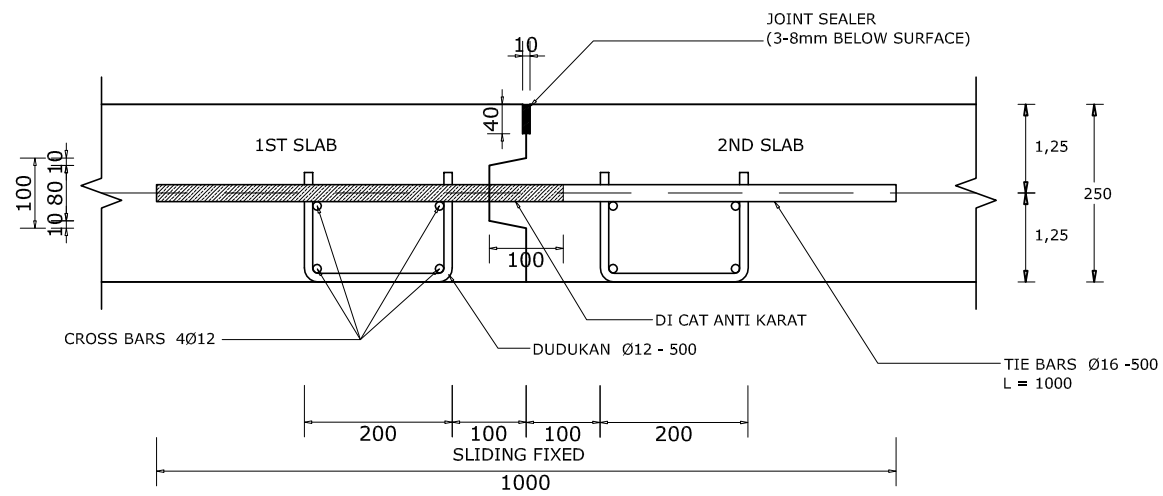
CONSTRUCTION JOINT MEMANJANG SKALA 1:10
