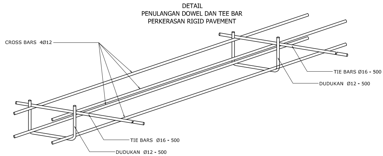
SUPPORT METHOD FOR TIE BARS SKALA 1:10
