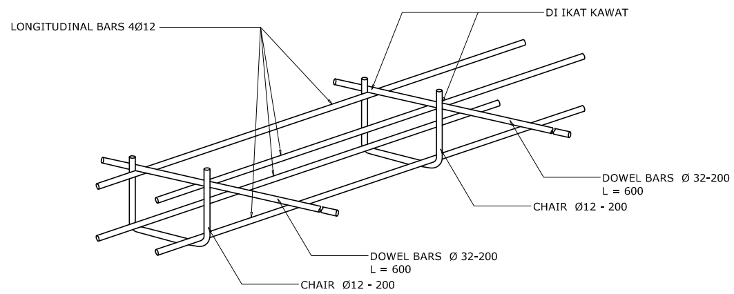
SUPPORT METHOD FOR DOWEL SKALA 1:10
